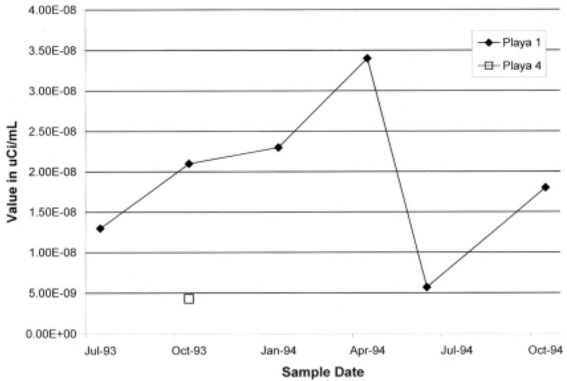
Beta Radiation
