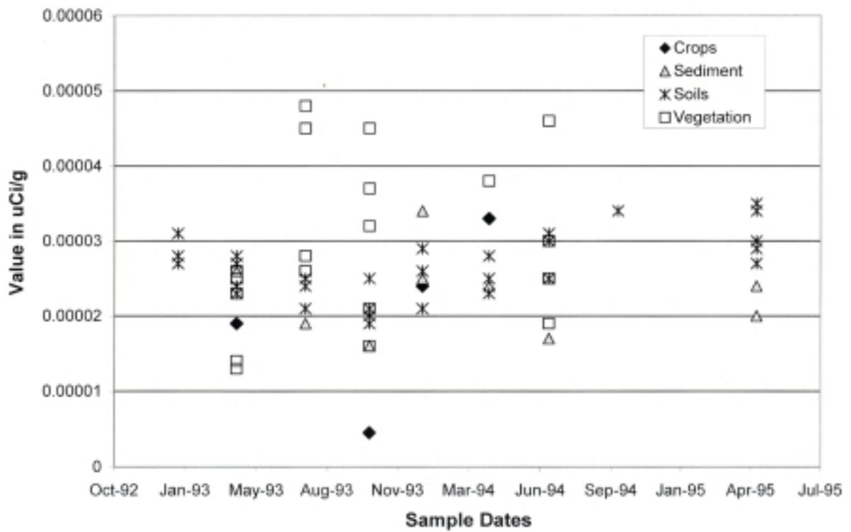
Beta Radiation
