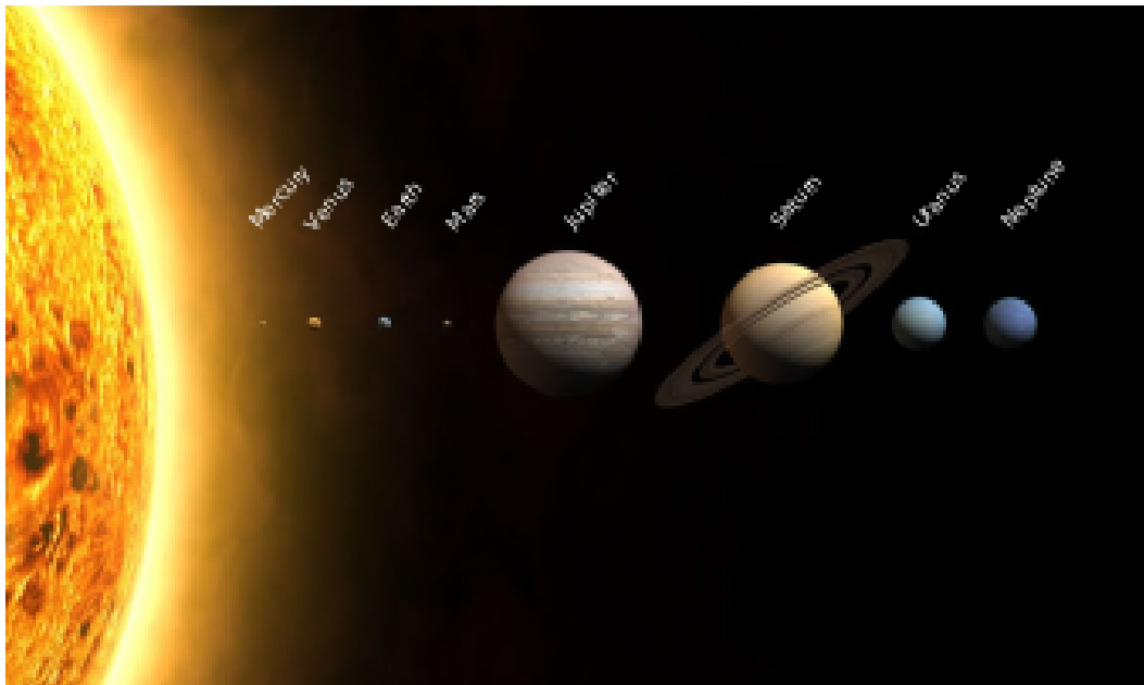
Figure 3.3: This figure shows the relative sizes of the planets. Closest to the Sun are the relatively small terrestrial planets, Mercury, Venus, Earth and Mars, composed of metals and rock. Farther out are two gas giants, Jupiter and Saturn, which are composed mainly of hydrogen and helium. Still farther out are two ice giants, Uranus and Neptune, which are composed mainly of frozen water, frozen ammonia and frozen methane. The distances of the planets from the Sun shown in this figure are not realistic. The planetary orbits lie in roughly in the same plane, which is called the ecliptic, and all the planets circle the Sun in the same direction.
