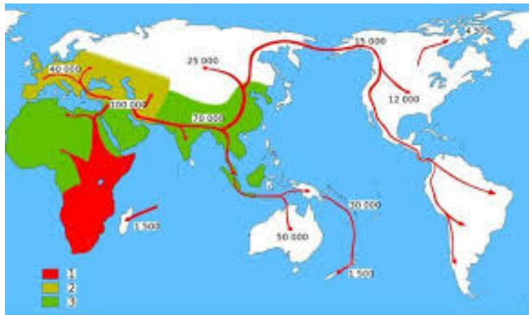
Figure 4.9: The spread of Homo sapiens
