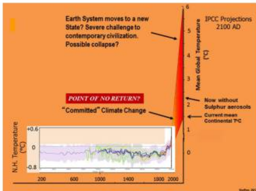
Figure 10.14: Historical and predicted global temperatures.
