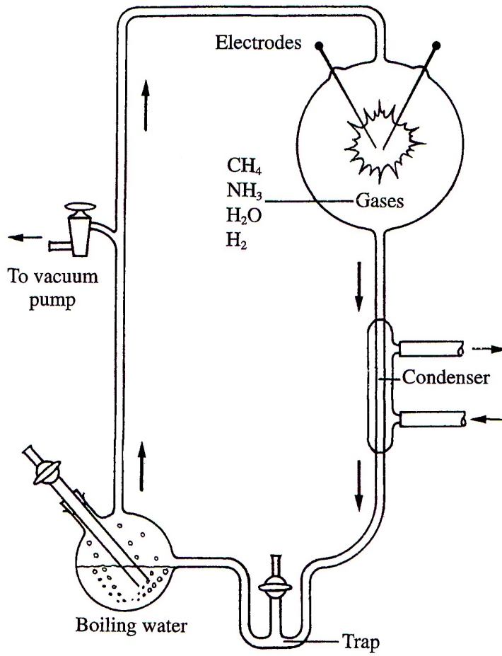
Figure 3.4: Miller's apparatus.
