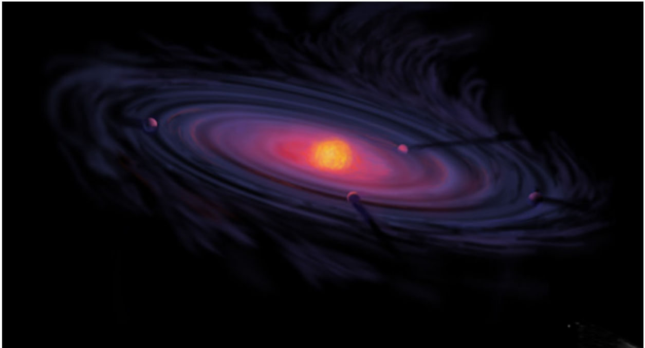
Figure 2.3: Artist's conception of a protoplanetary disc.
