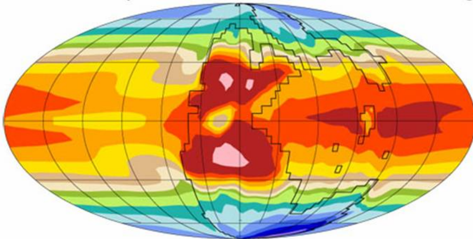
Permian (250Ma) Surface Temperature C
